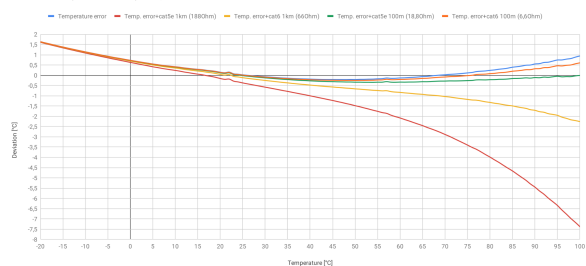
Temperature deviation for air sensor
